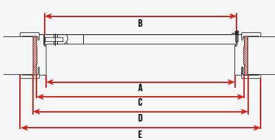
RESİM/PICTURE 1: KAPI GENEL KESİT DOOR'S GENERAL CROSS SECTION
